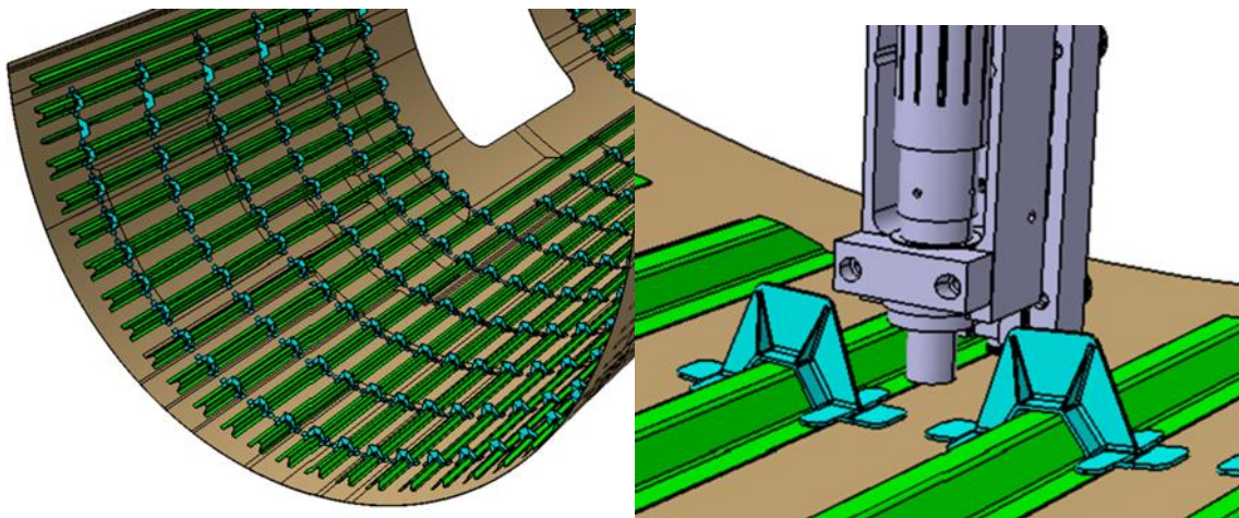
Figure 2: Stringers and clips welded to a thermoplastic fuselage
