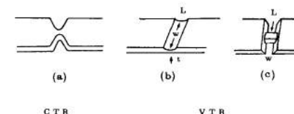
Figure 7.10 Different thin film bridge structures. (a) Constant thickness bridge (C.T.B.) or "Dayem bridge". (b), (c) variable thickness bridges (V.T.B.).
