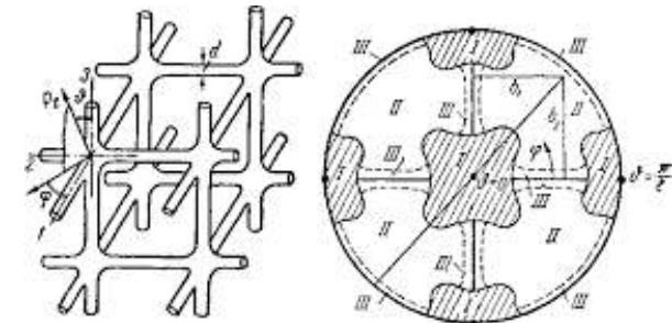
FIG. 2. Constant-energy surface of the "three-dimensional grid" type.
